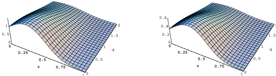
Figure 8.1: Probability distribution \Phi^I(z, \mathbf{q}_\perp) that three valence quarks leave the fraction z of the baryon momentum and transverse momentum \mathbf{q}_\perp to the quark-antiquark pair(s) in the vector I = V (left) and magnetic I = M (right) cases plotted in units of M and normalized to \Phi^V(0, 0) = 1 .
