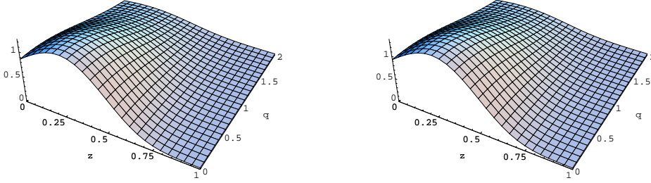
Figure 7.1: Probability distribution \Phi^I(z, \mathbf{q}_\perp) that three valence quarks leave the fraction z of the baryon momentum and transverse momentum \mathbf{q}_\perp to the quark-antiquark pair(s) in the axial I = A (left) and tensor I = T (right) cases plotted in units of M and normalized to \Phi^V(0, 0) = 1 .
