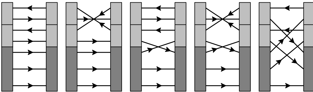
Figure B1: Schematic representation of the 7Q contributions to the normalization.
