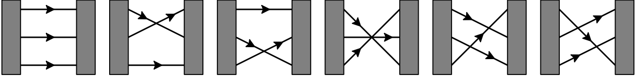
Figure 3.8: Schematic representation of the 3Q contribution to matrix elements. Each quark line stands for the color, flavor and spin contractions \delta_{\alpha'_i}^{\alpha_i} \delta_{f'_i}^{f_i} \delta_{\sigma'_i}^{\sigma_i} \int dz'_i d^2 \mathbf{p}'_{i\perp} \delta(z_i - z'_i) \delta^{(2)}(\mathbf{p}_{i\perp} - \mathbf{p}'_{i\perp}) with the primed variables referring to \Psi^{(3)\dagger}(B) (right rectangle) and the unprimed ones to \Psi^{(3)}(B) (left rectangle). A crossing of these quark lines corresponds to an anticommutation of two creation or annihilation operators and thus introduces a minus sign. This sign is however compensated by the one coming from the contraction of \epsilon tensors with color indices. Since only valence quarks are involved all those diagrams are equivalent to the first one.
